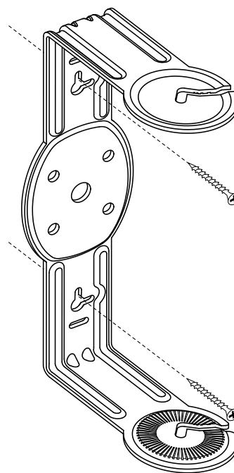
Mounting bracket vertical position
