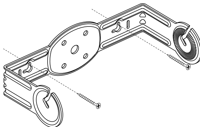
Mounting bracket horizontal position
