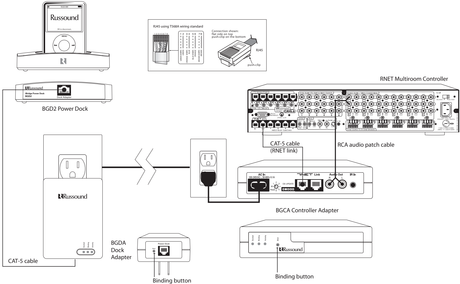
Typical installation for RNET multiroom controller system
