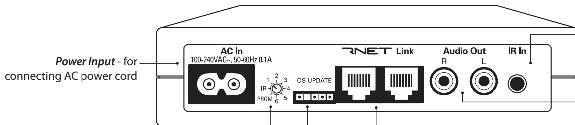
BGCA Controller Adapter (back)
