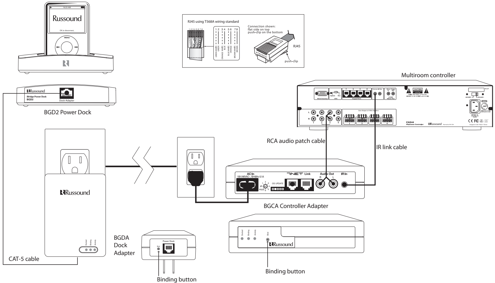
Typical installation for IR control multiroom controller system
