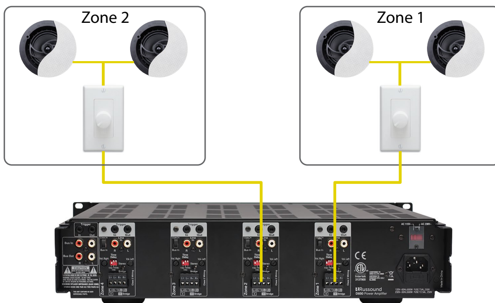
Connection diagram showing volume controls connected to D850 amplifier
