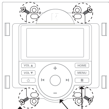
Mounting screws Plastic buttons/ring KLK-E6 without cover
