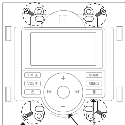
Mounting screws Plastic buttons/ring KLK-E5 without cover
