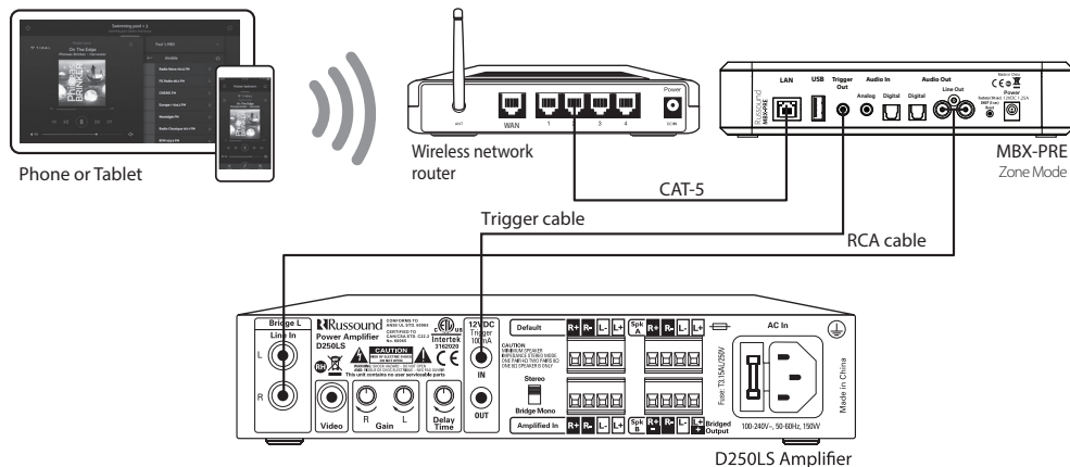
Connection with D250LS amplifier
