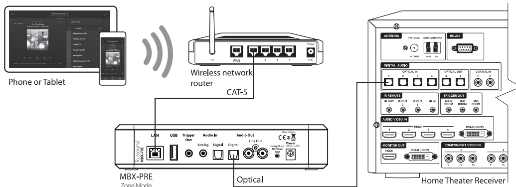
Connection with home theater receiver
