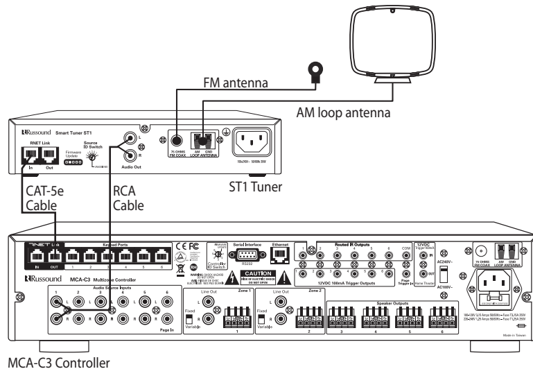
RNET Source Connection to MCA-C3
