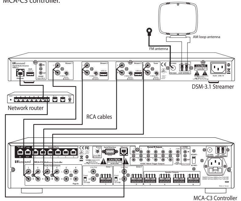
Audio Source Connection to MCA-C3
