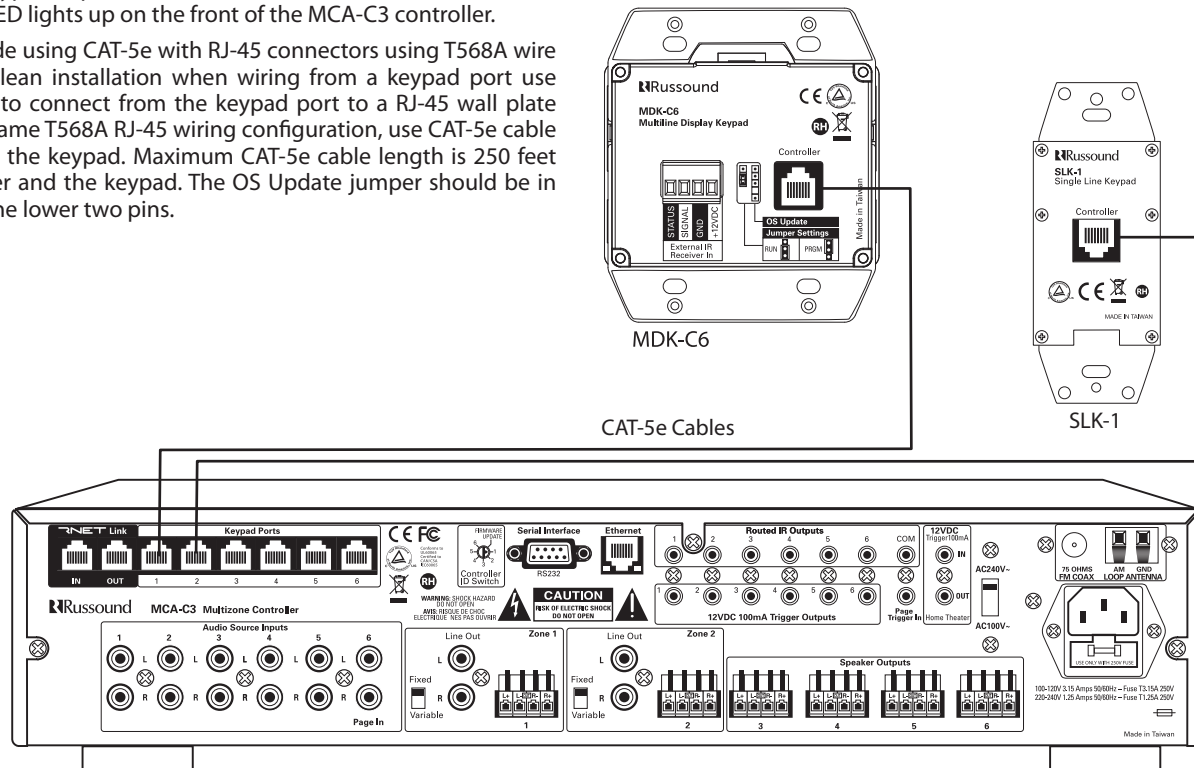
Keypad connection to the MCA-C3
