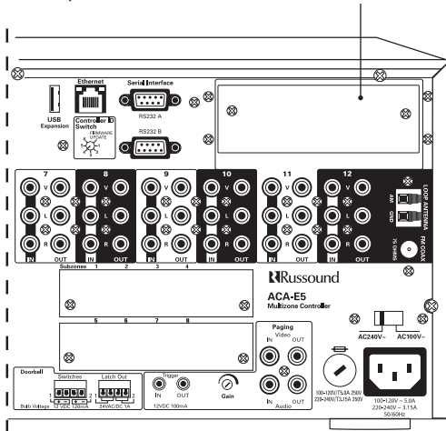
ACA-E5 rear panel location of module installation
