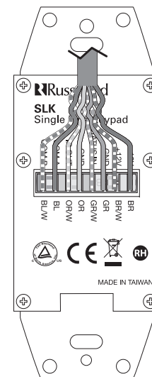
CAT-5 to SLK Connection
