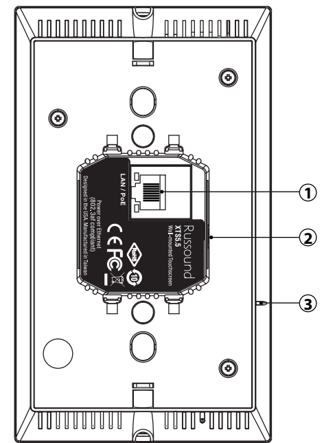
Back Panel
